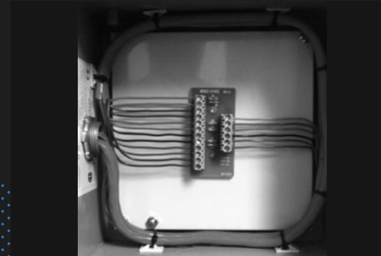
TYPICAL INSTALLATION*
